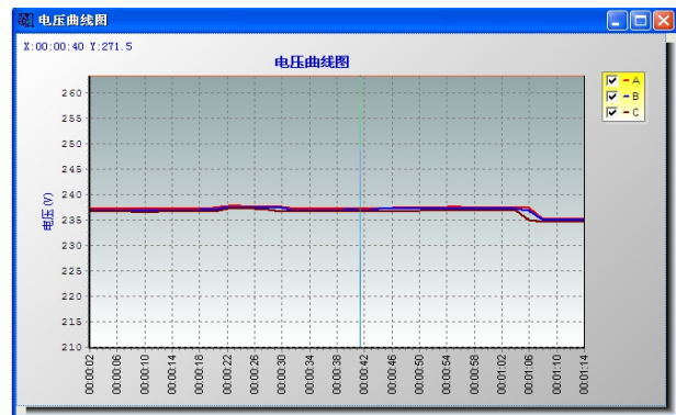
Voltage curve
